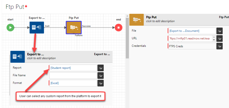
Screenshot: FTP Put implementation example
